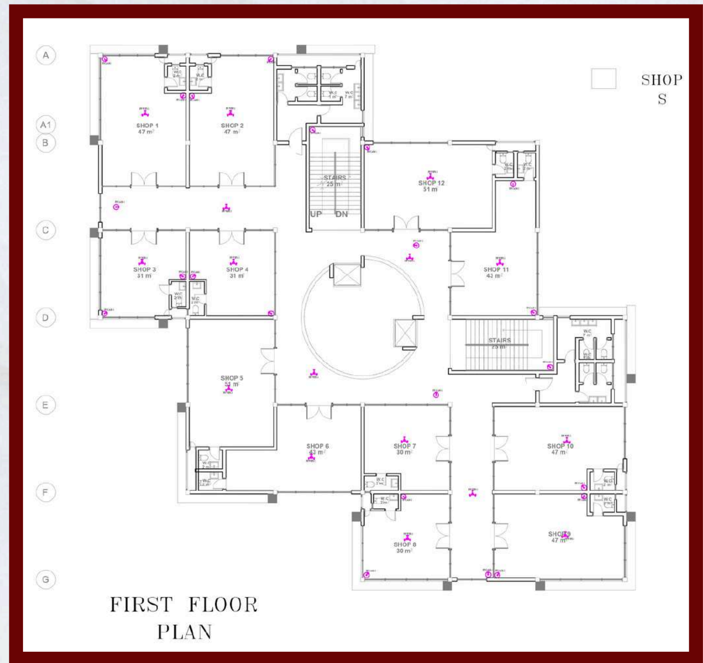
First Floor
